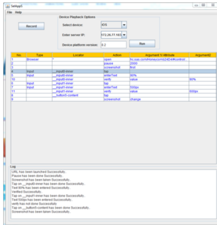
Figure 3: Running test case and log generation
